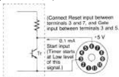
Solid-state circuit (proximity sensor, photoelectric sensor, etc.)
