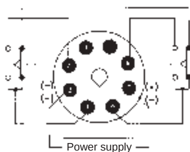
Without Reset Input (H3CR-H8L)
