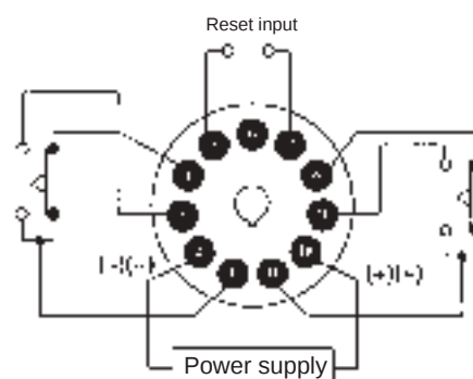
With Reset Input (H3CR-HRL)
