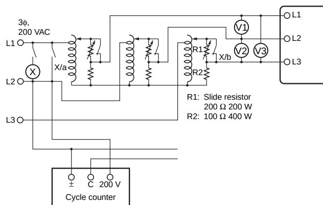
Connection Diagram
