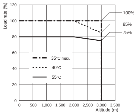
240 W/480 W/960 W &lt;Horizontal separation: less than 15 mm&gt;
