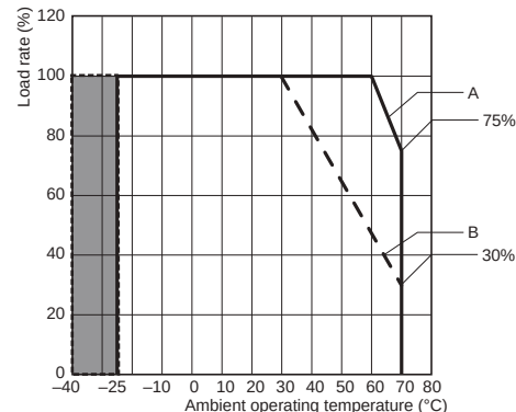
960 W &lt;Horizontal separation: 15 mm or more&gt;
